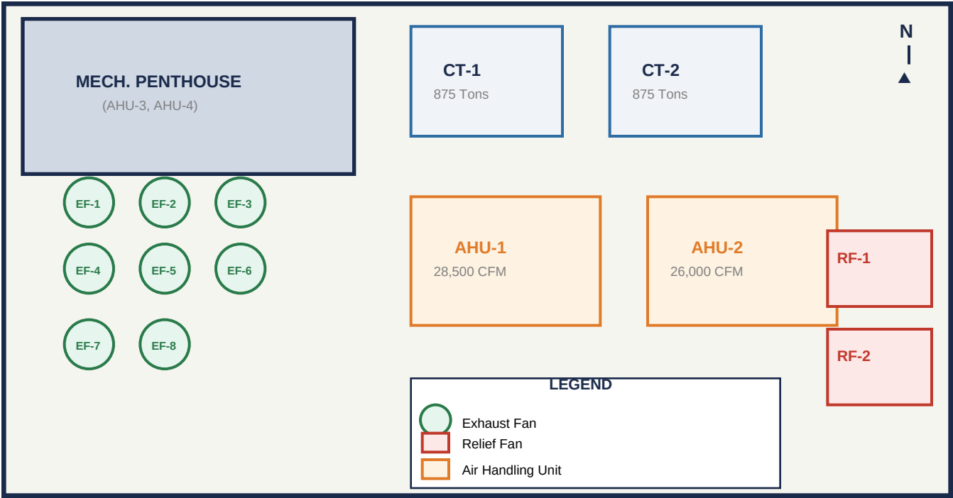
Figure 5 — Rooftop Mechanical Equipment Plan (Schematic — Not to Scale)
